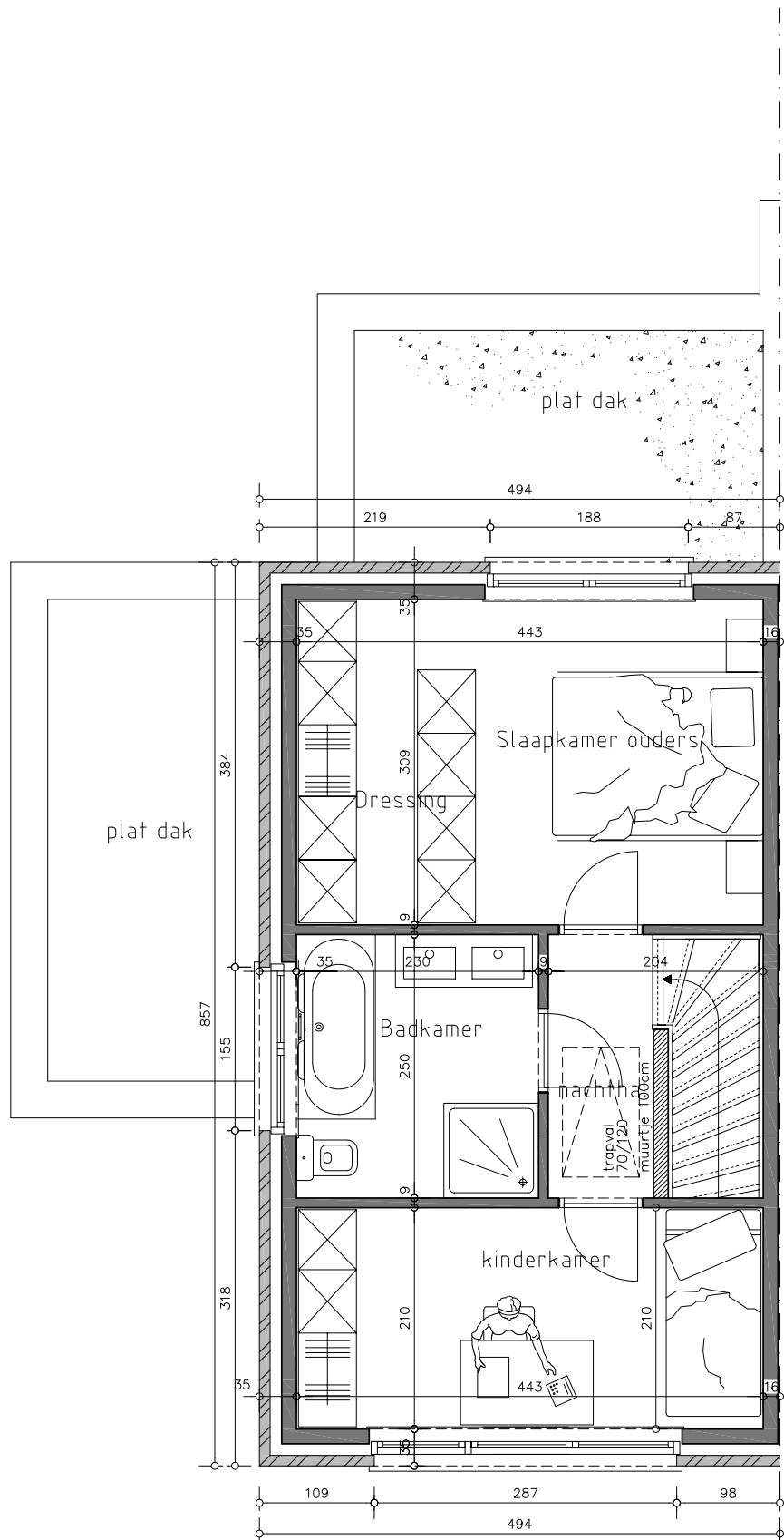
Verdieping VDL Opp: 42.34 m 2
